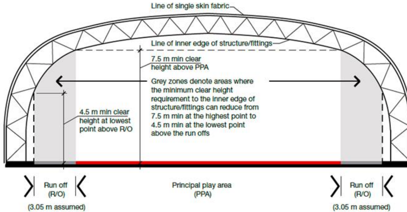
Generic covered outdoor court section showing minimum clear height requirements
